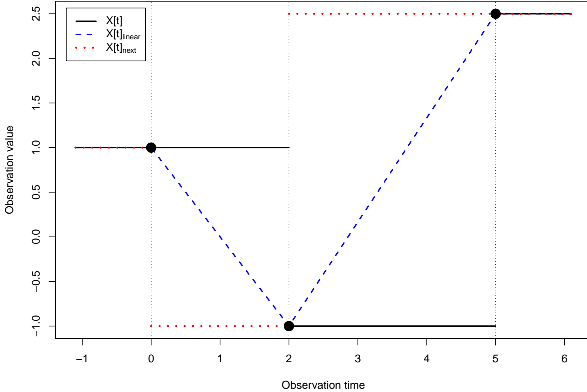
Figure 1: The sampling-scheme-dependent graph of the time series X with T(X) = (0, 2, 5) and V(X) = (1, -1, 2.5) . The three observation time-value pairs are denoted by solid black circles.
